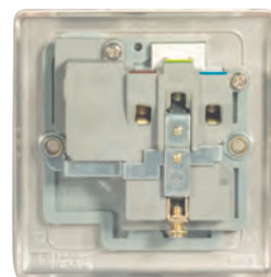
Angled in-line colour coded captive terminals
